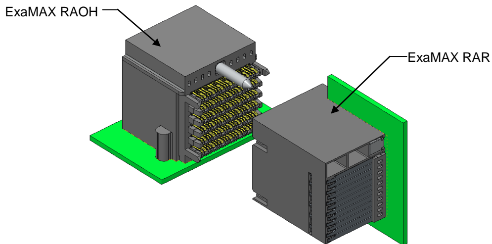
RIGHT ANGLE ORTHOGONAL HEADER (RAOH) WITH RIGHT ANGLE RECEPTACLE (RAR) (6-Pair, 12-Column Configuration with Guides Shown)
