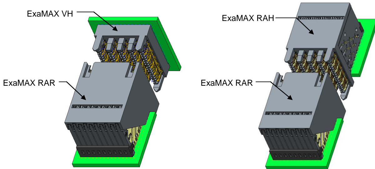
BACKPLANE RIGHT ANGLE RECEPTACLE (RAR) AND VERTICAL HEADER (VH) COPLANAR RIGHT ANGLE RECEPTACLE (RAR) AND RIGHT ANGLE HEADER (RAH) (4-Pair, 10-Column Configuration Shown)
