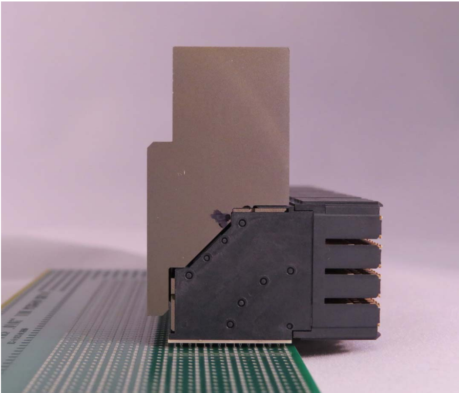
Figure 6: Proper 4 Pair loading head with a 4 pair connector.
