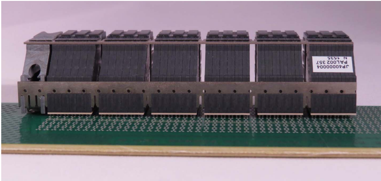
Figure 5: Rear view of the assembly. Check for bent pins.
