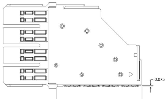
Figure 8: 0.075 mm maximum height off board surface
