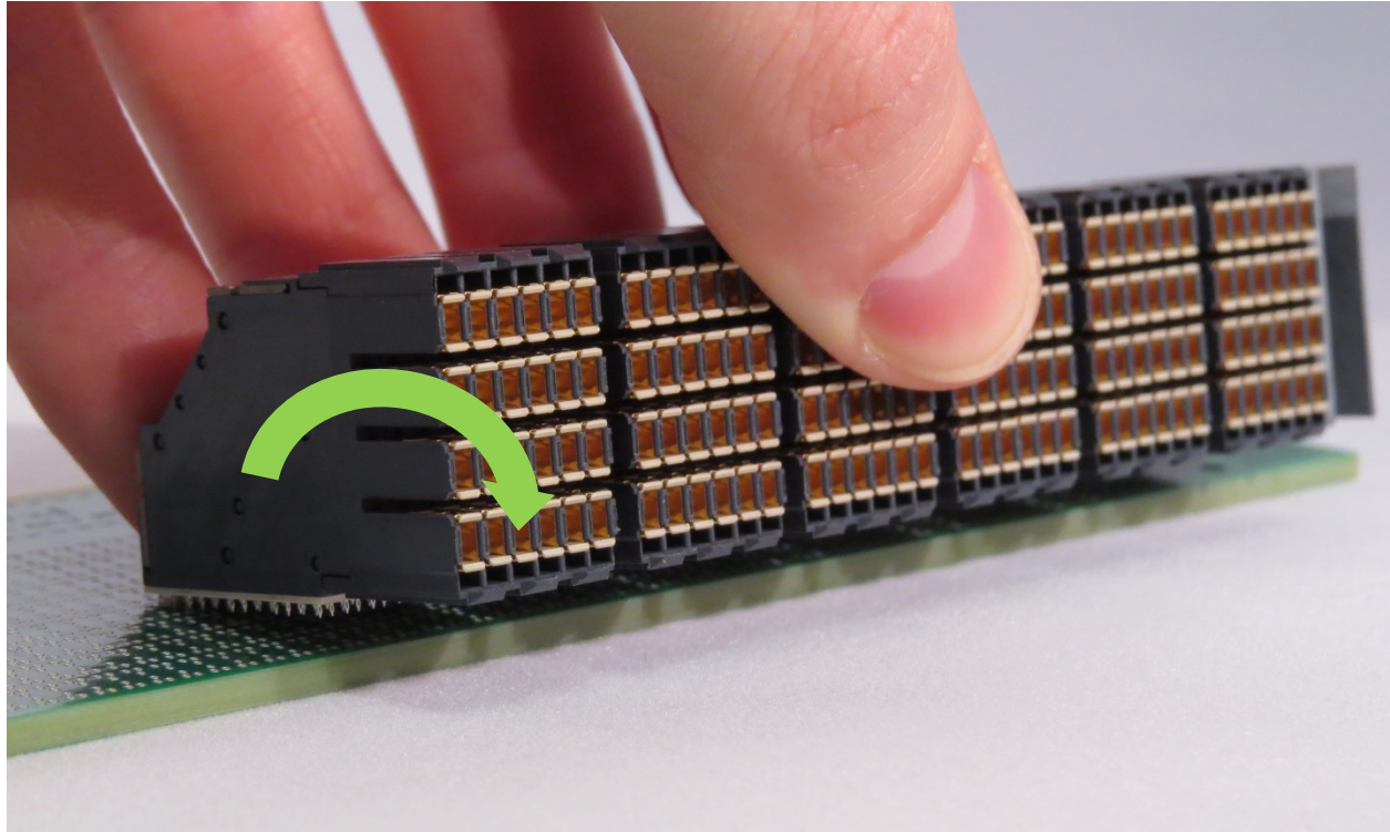
Figure 3: With the back row entirely placed, roll connector toward board edge placing the remaining rows of compliant pins.
