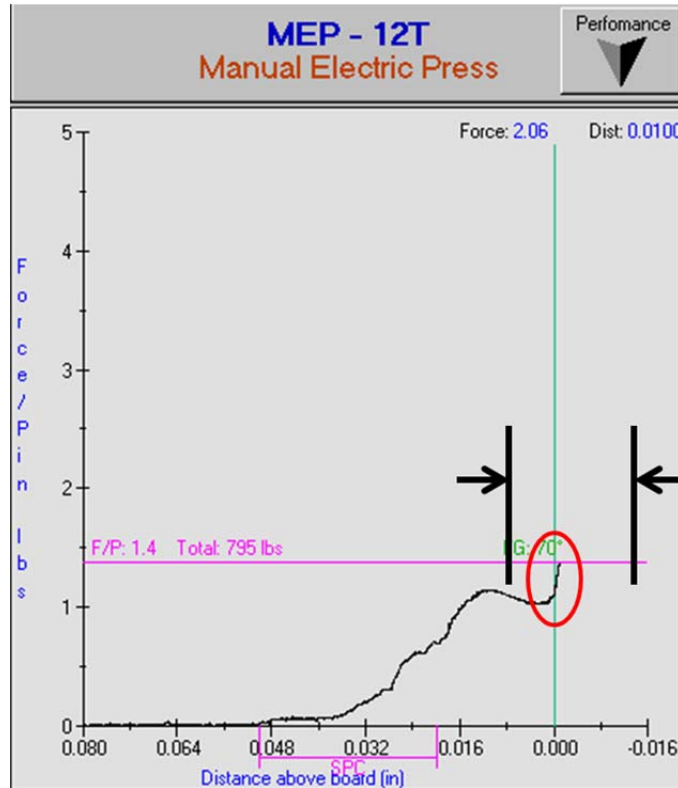
Figure A-10. Press sequence force gradient termination.
