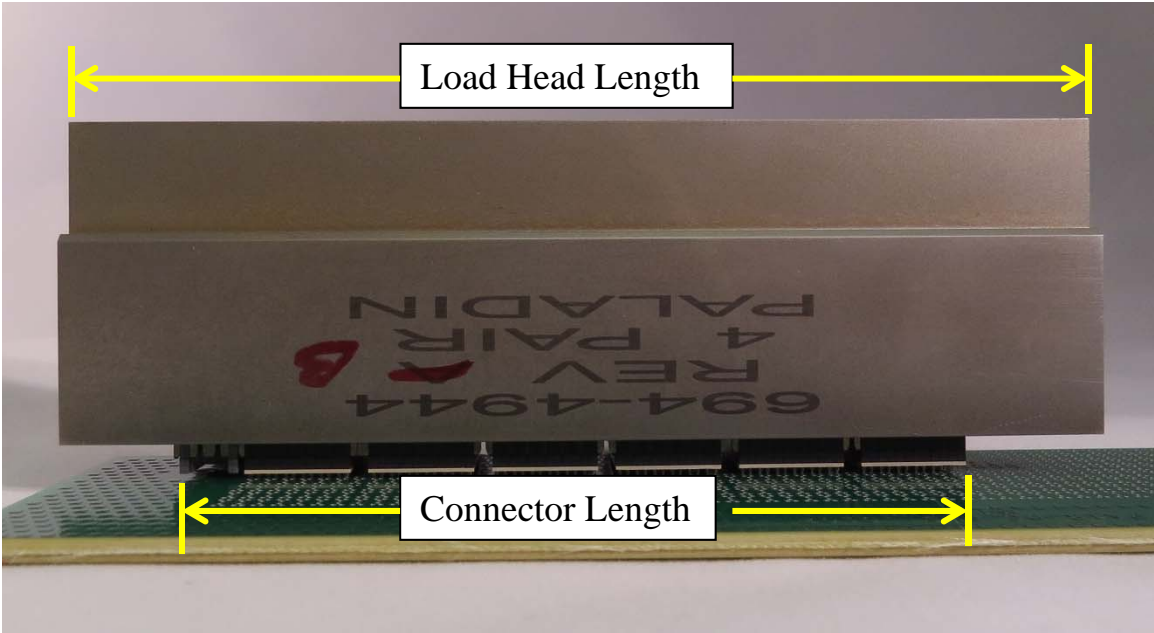
Figure 7: Ensure that the load head length is equal to or greater than the connector length.
