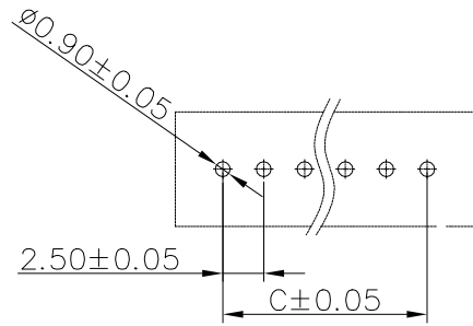
RECOMMENDED PCB LAYOUT PCB THK=1.6±0.05
